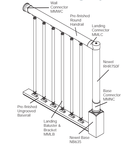
Landing or horizontal balustrading only
