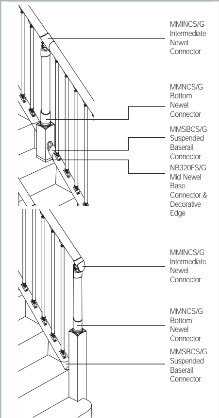
Staircase configurations with cut string option
