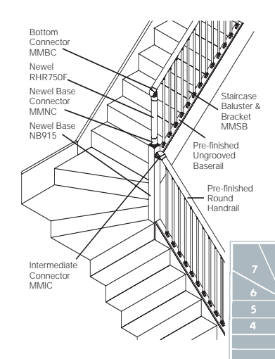
Quarter turn with 3 winders
