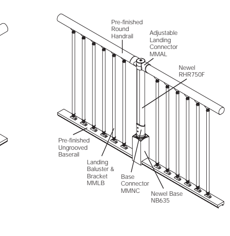
Continuous rail over newel
