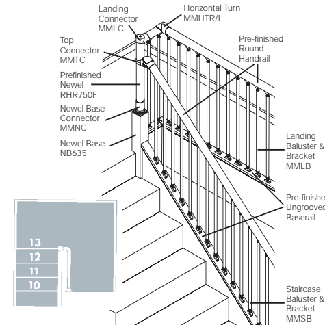
Top landing, 180° turn with winders
