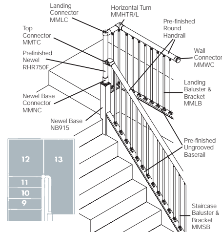
Top landing with 180° turn
