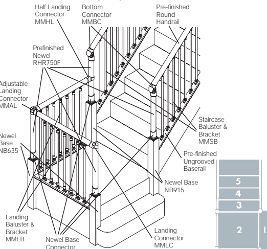
Half turn with extended landing
